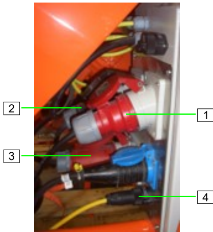
Abb. 30: Stromanschlüsse
